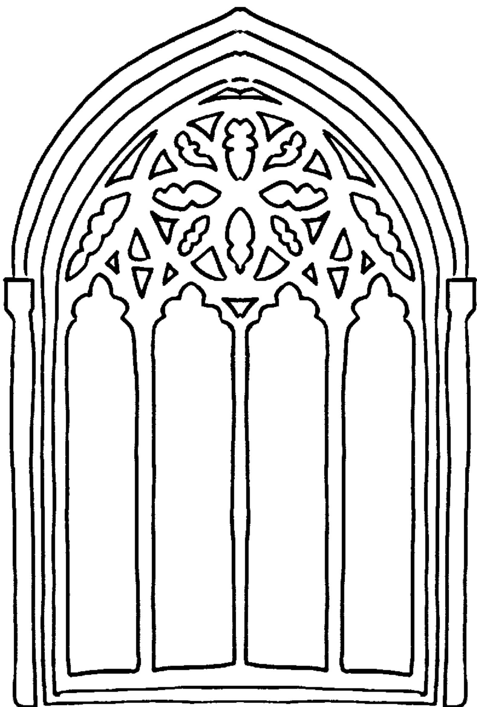
Decorated
