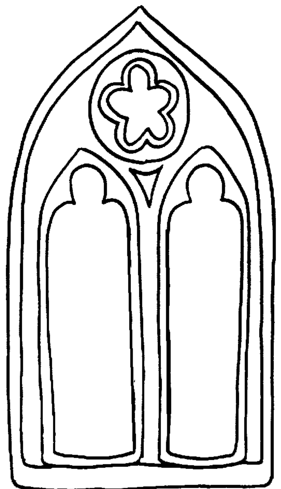
Victorian Gothic
