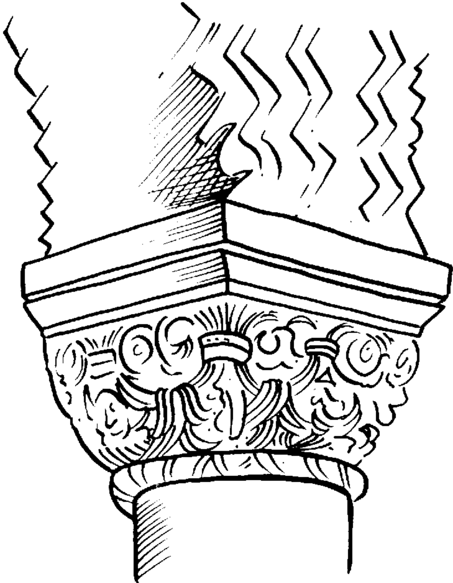
Late Norman
