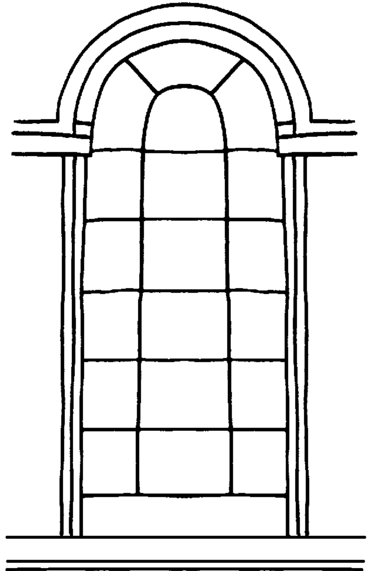
Regency Window
