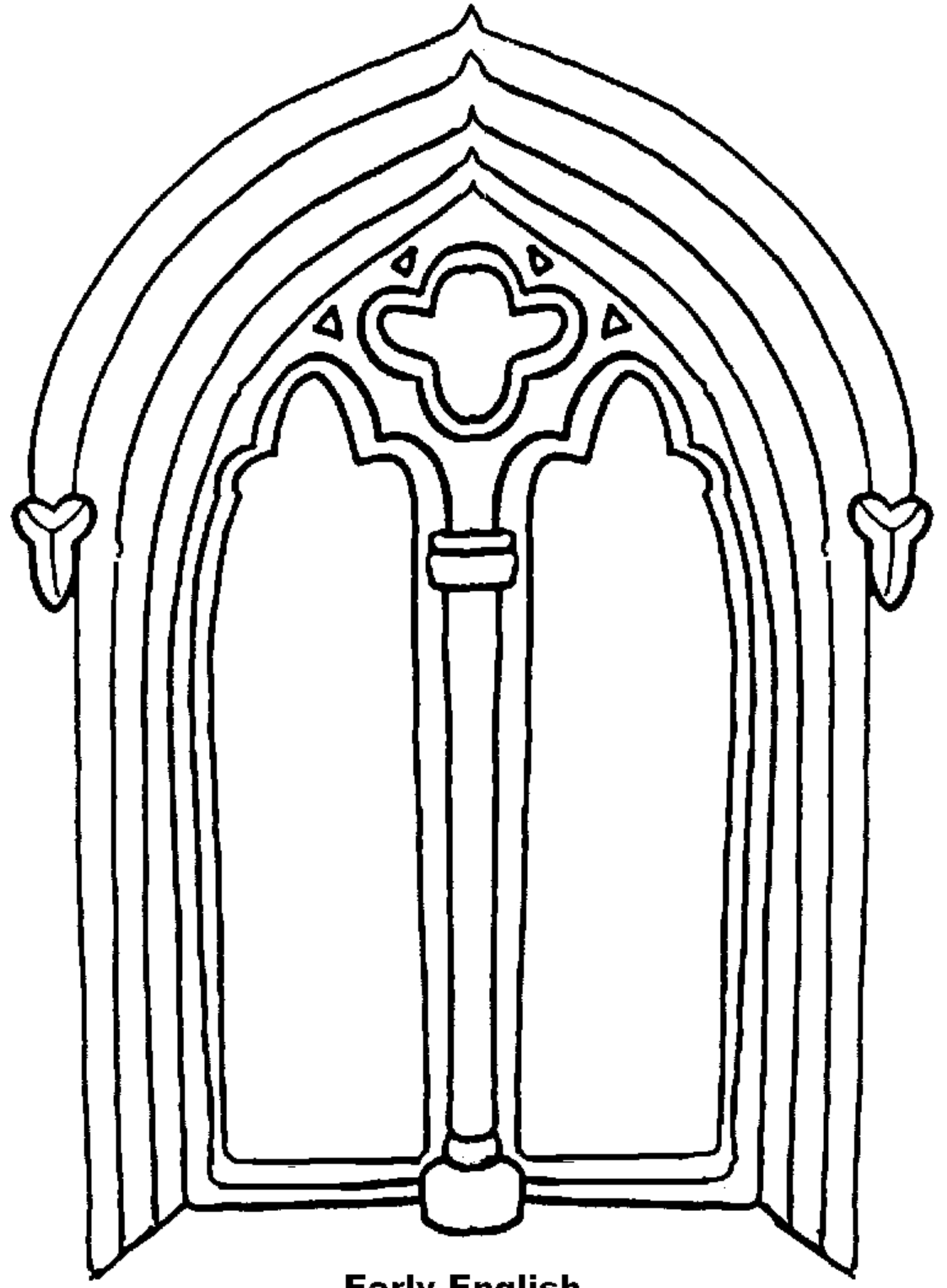
Early English
