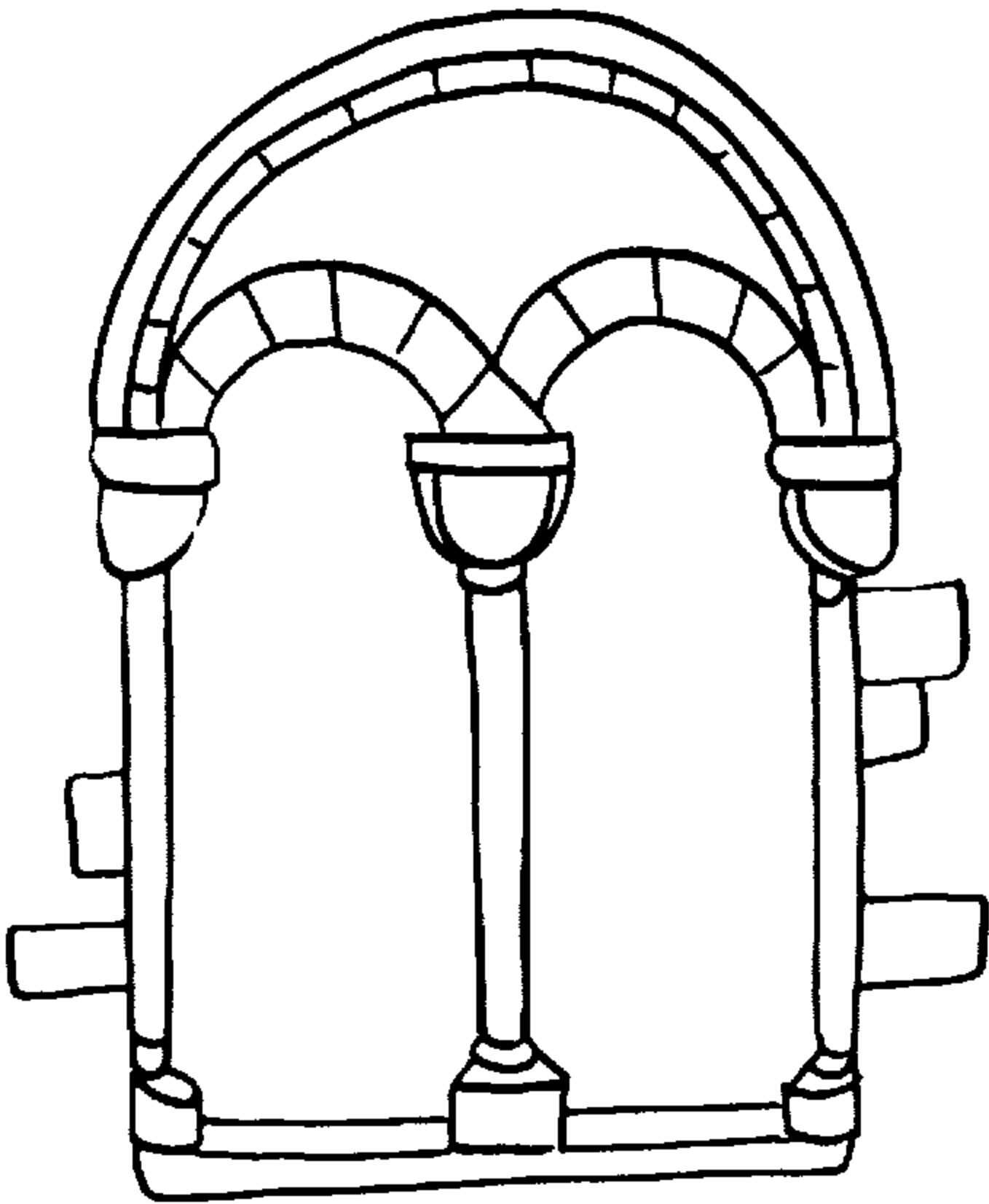
Norman
