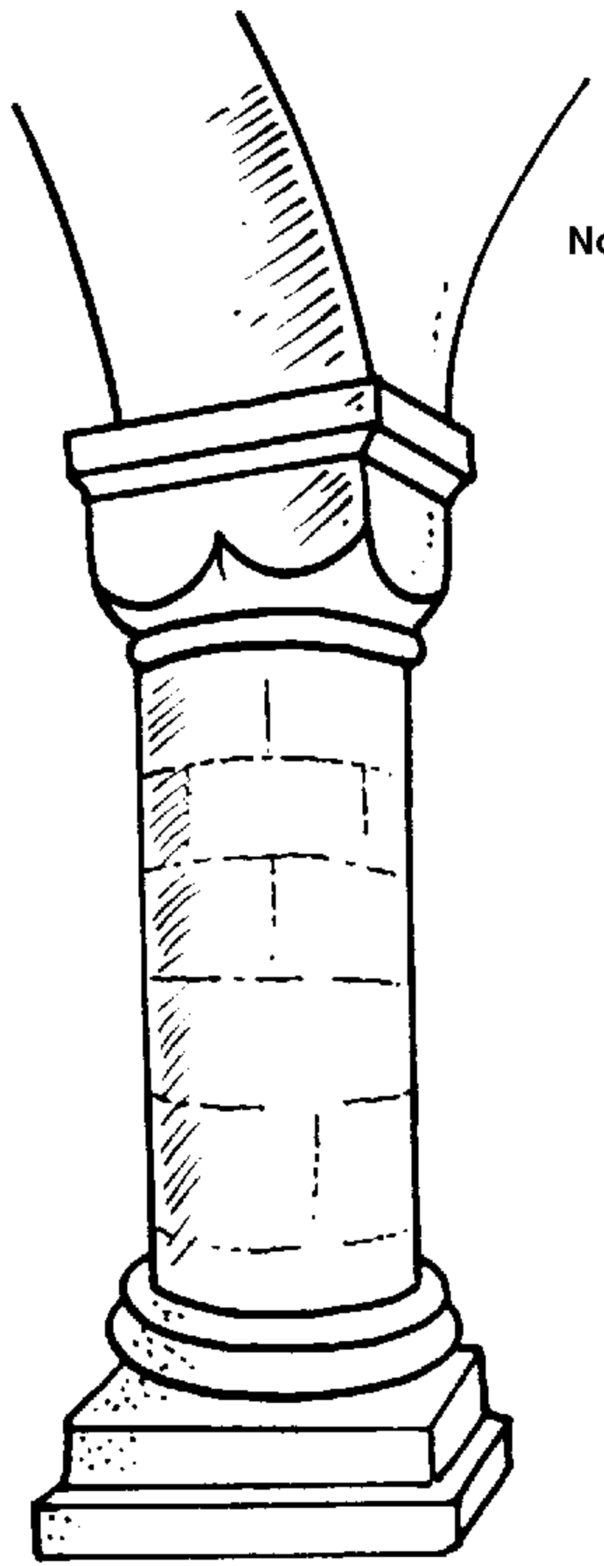
Late Norman
